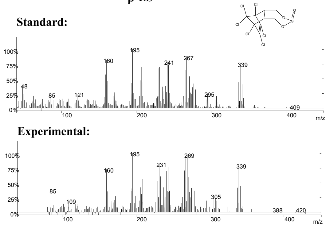
Sup. Figure 3. Mass spectra of \beta -ES.
